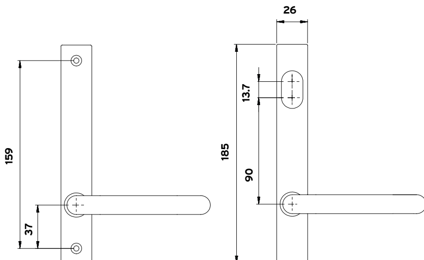
N100 Plate with lever - concealed
