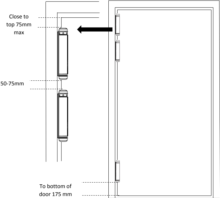
Single Door Installation
