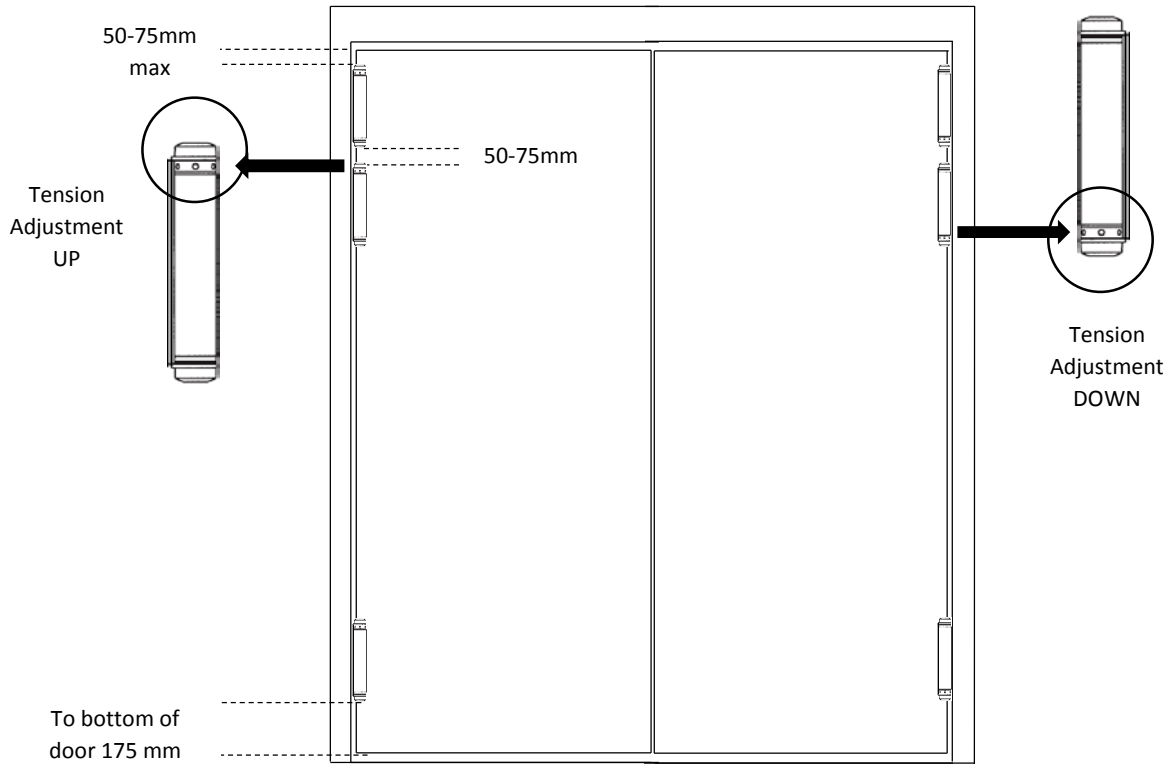
Double Door Installation
