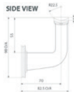
Showing flat mount adaptor
